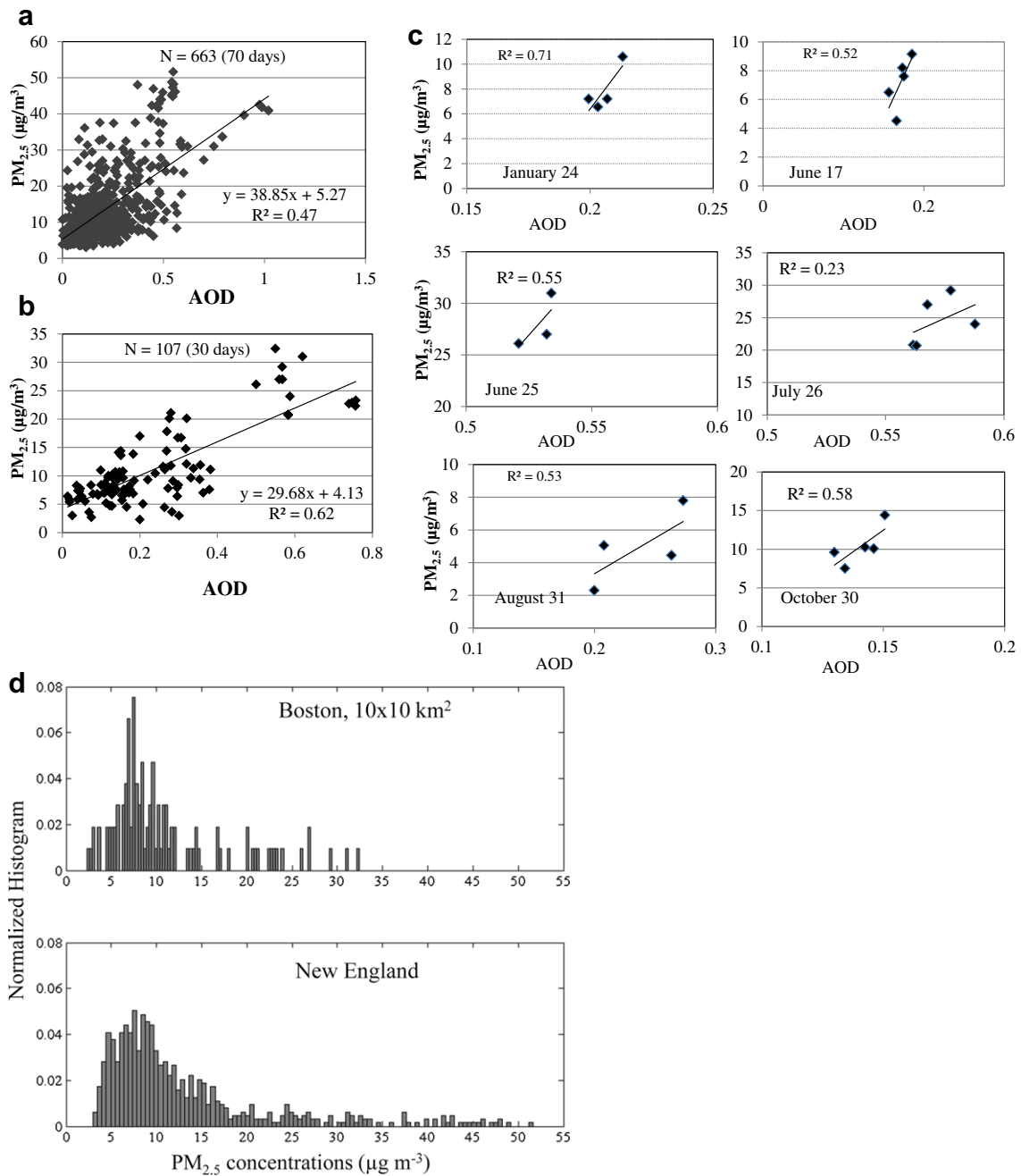
Fig. 3. Left panel: Regional (a) and Intra-urban (b) 1 km AOD-PM 2.5 correlation for 2003. Right panel (c): Examples of intra-urban daily correlation between 1 km AOD and PM 2.5 for six different days. Note up to 10 \mu\text{g m}^{-3} variability in PM 2.5 between EPA monitoring stations. (d): Normalized histogram of PM 2.5 concentrations for Boston ( 10 \times 10 \text{ km}^2 box, top) and New England (bottom) domains.
