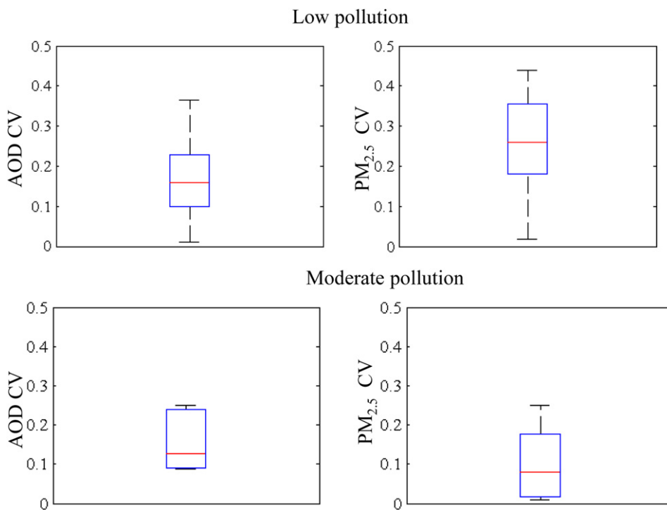
Fig. 7. AOD coefficient of variation (CV) and PM_{2.5} CV calculated for the 10 \times 10 km^2 area. Upper panel: low pollution days ( PM_{2.5} < 15 \mu g m^{-3} ); Lower panel: moderate pollution days ( PM_{2.5} > 15 \mu g m^{-3} ).
