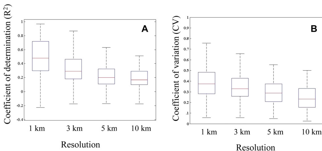
Fig. 5. A: Coefficient of determination ( R^2 ) for \text{PM}_{2.5} , measured by the EPA ground-monitoring stations, and MAIAC retrieved AOD as a function of spatial resolution. The correlation deteriorates as imaging resolution coarsens towards the conventional 10 km. Red line represents the median value, the edges of the box are the 25th and 75th percentiles, the whiskers indicate the range. B: AOD coefficient of variation (stdev divided by the mean) also decreases with the coarsening resolution. (For interpretation of the references to color in this figure legend, the reader is referred to the web version of this article.)
