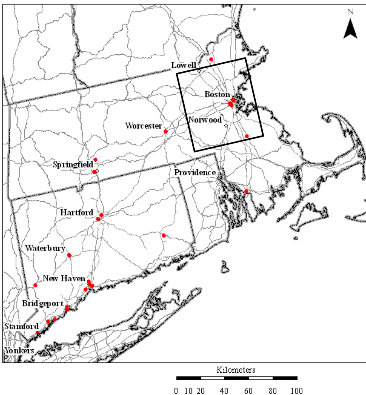
Fig. 1. Study area. The dots mark locations of the EPA PM_{2.5} ground monitoring sites. The area highlighted by rectangle shows the 60 \times 70 \text{ km}^2 Boston metropolitan area.
