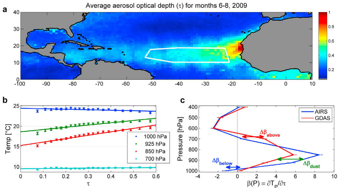
Figure 1. Detecting the radiative signal of transatlantic dust. (a) Mean aerosol optical depth ( \tau ) for the summer months (June–August), 2009. The dust plume region is clearly visible. The white line delimits the study region. (b) Observed (binned) temperature at four pressure levels versus \tau , for the region shown in Figure 1a. Each point is an average of \sim 280 pixels, and the average is within the error-bars at 99% confidence level. The straight lines are linear fits. (c) Vertical profiles of \beta(P) \equiv \partial T_p / \partial \tau ; positive values of \beta indicate heating. Observe a cooling of \sim 1 K per unit \tau at a pressure level of 1000 hPa (below the dust layer), heating of \sim 6 – 8 K per unit \tau at 925–850 hPa (within the dust layer), and cooling of \sim 2 K per unit \tau at 600–500 hPa (above the dust layer). The blue curve was calculated using observed temperature profiles (from AIRS), while the red curve uses modeled data (from GDAS). The error bars indicate the 99% confidence region. The differences between the two curves serve as lower bound for the dust radiative signature: cooling below the dust layer, heating within it, and cooling above it ( \Delta\beta \equiv \beta_{\text{obs.}} - \beta_{\text{modl.}} < \beta_{\text{total}} - \beta_{\text{meteorology}} < \beta_{\text{dust}} ).
