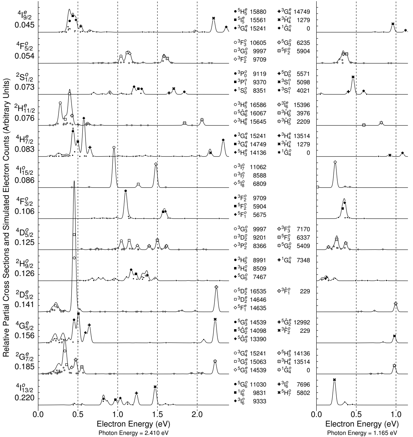
FIG. 2: Simulated electron counts and relative partial cross sections for given \text{Ce}^- initial states (continued, see Fig. 1).
