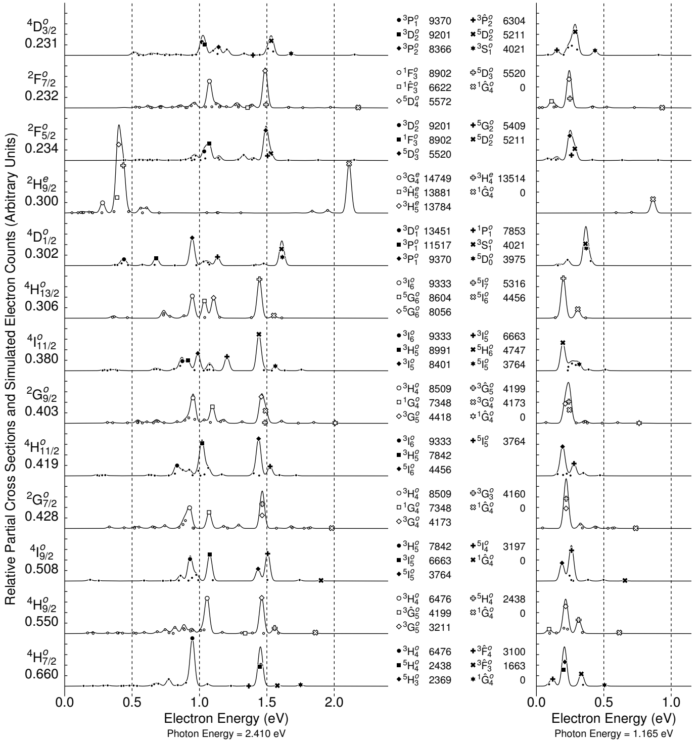
FIG. 1: Simulated electron counts and relative partial cross sections for given \text{Ce}^- initial states. The dominant LS term and binding energy (in eV) for each odd ( 4f5d^26s^2 ) or even ( 4f5d6s^26p ) \text{Ce}^- level appear on the left side of each row. The legend for each row indicates the most important channels by corresponding neutral Ce threshold (with energy in \text{cm}^{-1} [5]), mainly 4f5d^26s/4f5d6s6p for odd/even levels with “ ^o ” in the LS term indicating 4f5d6s^2/4f^25d6s levels.
