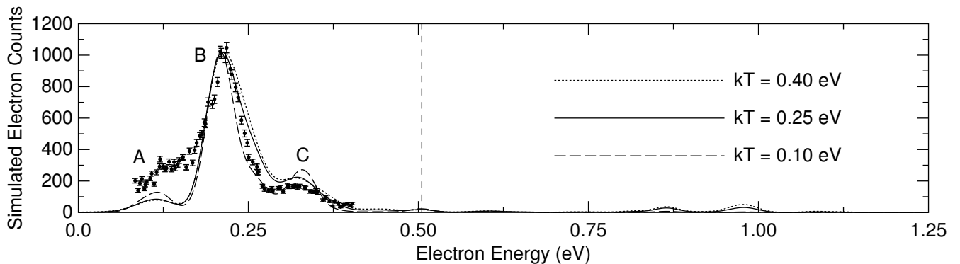
FIG. 4: Simulated electron counts for incident photon energy of 1.165 eV. The points and error bars are the Davis and Thompson [10] experimental results. The dashed vertical line indicates the position of the ground state to ground state channel with our revised interpretation.
