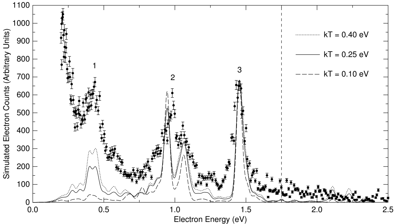
FIG. 3: Simulated electron counts for incident photon energy of 2.410 eV. The points and error bars are the Davis and Thompson [10] experimental results. The dashed vertical line indicates the position of the ground state to ground state channel with our revised interpretation. The broad low energy increase in electron counts in the experimental data is due to “collisional detachment of Ce^- ions in the beam by background gas and ion-aperture scattering” and has not been included in our simulated plots.
