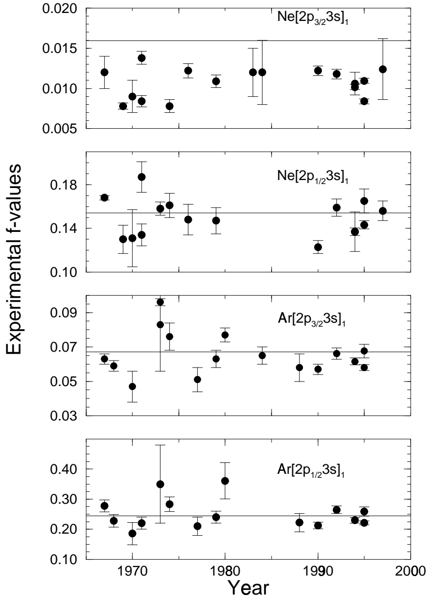
FIG. 1. Experimental f-values for the [2p_{3/2}^{-1}3s_{1/2}]_1 and [2p_{1/2}^{-1}3s_{1/2}]_1 states of Neon and the [3p_{3/2}^{-1}4s_{1/2}]_1 and [3p_{1/2}^{-1}4s_{1/2}]_1 states of Argon. The horizontal lines refer to the average of our calculated f-values in length and velocity forms.
