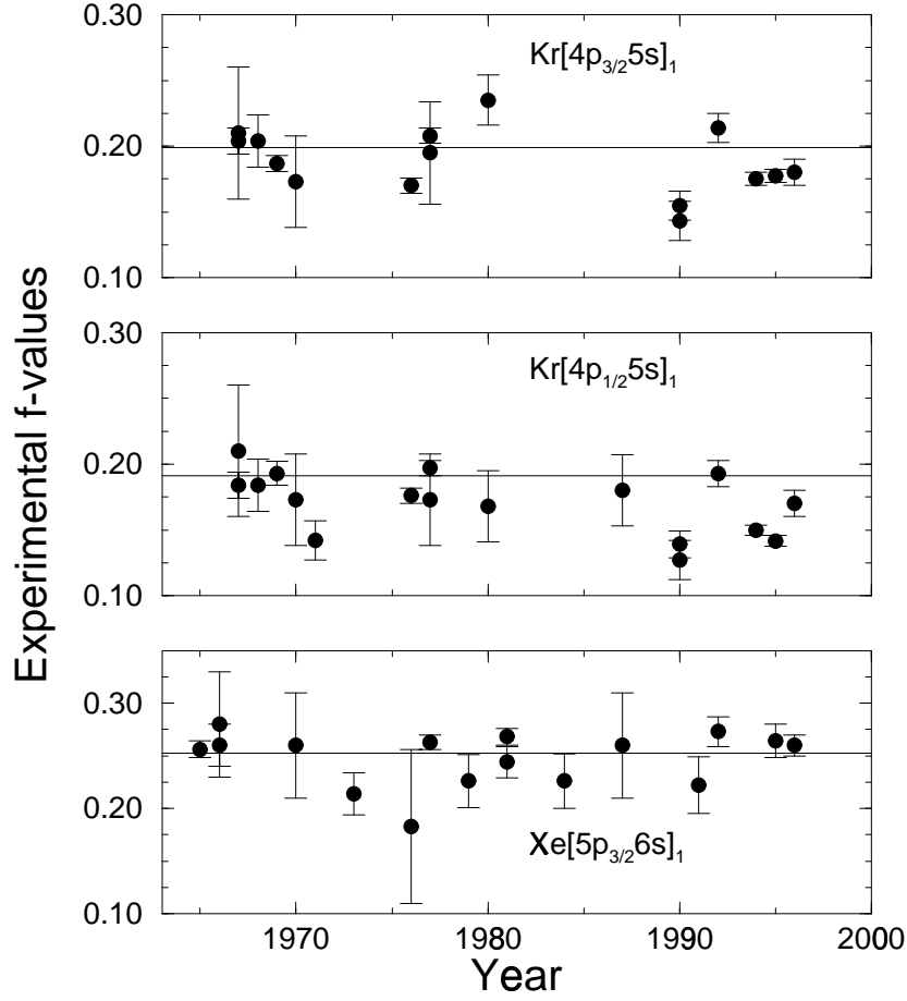
FIG. 2. Experimental f-values for the [4p_{3/2}^{-1}5s_{1/2}]_1 and [4p_{1/2}^{-1}5s_{1/2}]_1 states of Krypton and the [5p_{3/2}^{-1}6s_{1/2}]_1 state of Xenon. The horizontal lines refer to the average of our calculated f-values in length and velocity forms.
