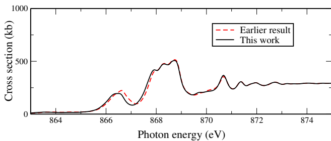
FIG. 2: (Color online). Calculated x-ray absorption cross section of atomic neon, near the Ne K edge, in the presence of an 800-nm laser field at an intensity of 10^{13} W/cm ^2 . The laser and x-ray polarizations are assumed to be linear and parallel to one another. The data indicated by the label “Earlier result” were calculated using the input data underlying Ref. [7]. In the present work, the energy splitting between the 3s and 3p orbitals was adjusted to coincide with the energy splitting between 1s^{-1}3s\ ^1S_0 and 1s^{-1}3p\ ^1P_1 calculated in Sec. II.
