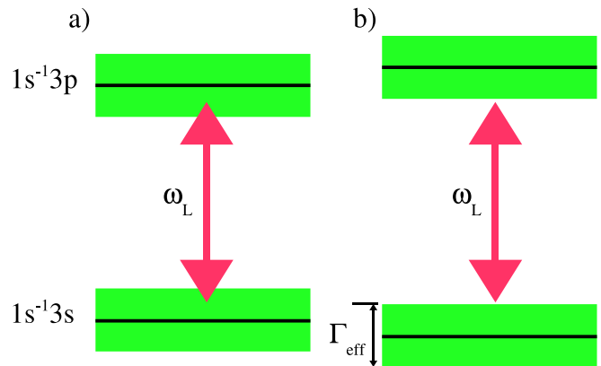
FIG. 1: (Color online). The laser photon energy \omega_L is kept fixed. (a) One possibility is that the true energy splitting between the 1s^{-1}3s\ ^1S_0 and 1s^{-1}3p\ ^1P_1 states agrees with \omega_L to within the decay width \Gamma_{\text{eff}} . (b) Another possibility is that the transition between 1s^{-1}3s\ ^1S_0 and 1s^{-1}3p\ ^1P_1 is not in resonance with \omega_L .
