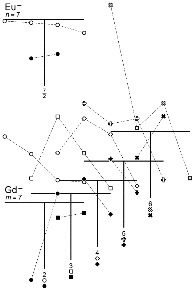
FIG. 2: Patterns of 6p attachments to neutral states, \text{Eu}^- 4f^7 6s^2 6p [2] versus \text{Gd}^- 4f^7 5d 6s^2 6p . The crossbar of the T-shaped representation of the neutral thresholds indicates the J range of 6p attachments ( J increasing to the right), and the stem gives the position of the neutral J and the vertical energy scale (200 meV). The number at the bottom of each stem gives the neutral J and, in the Gd case, the symbols associated with that neutral level. The full and open symbols represent anion 6p_{1/2} and 6p_{3/2} attachments to those levels, respectively.
