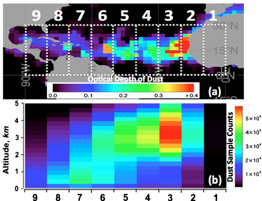
Figure 2. (a) Positioning of the nine consecutive regions studied along the typical summertime track of Saharan dust. Colors encode values of the median optical depth of dust layers at 2° by 2° horizontal resolution. (b) Vertical distribution of the number of 5 km-resolution dust samples in the nine regions. Each bin has a height of 270 m.
