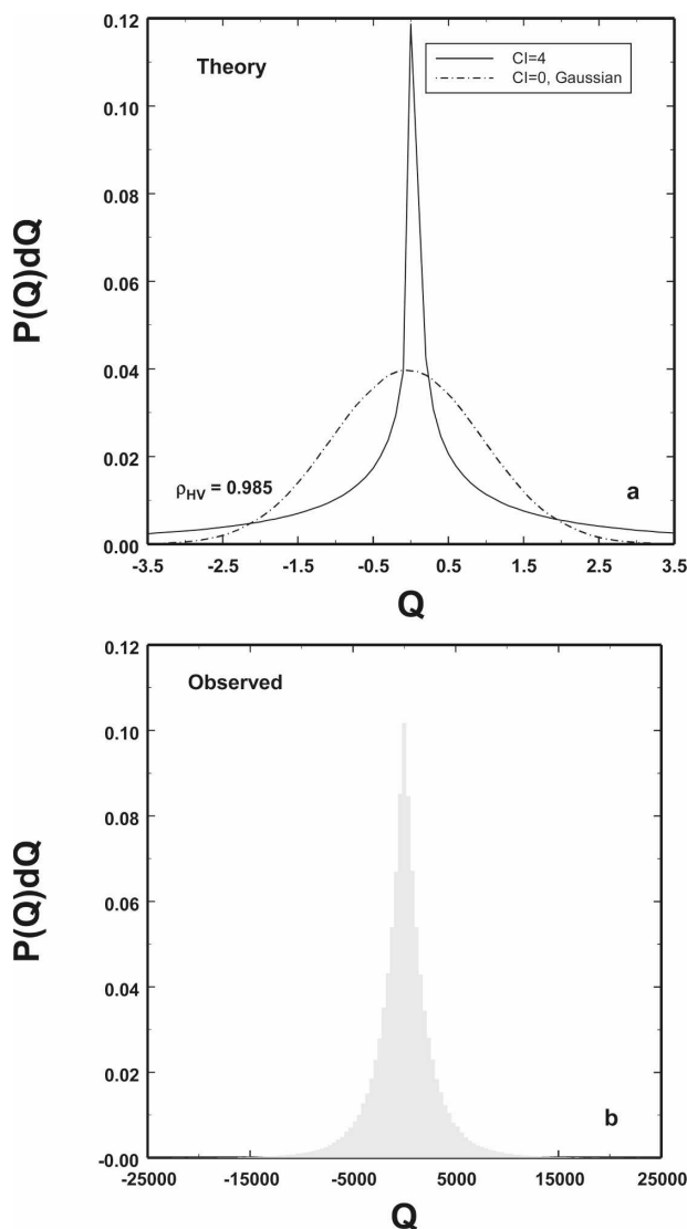
FIG. 3. (a) Frequency distributions for the Q component of the complex amplitude for Rayleigh signal statistics (the Gaussian distribution) and simulated clustered case for the same mean I as discussed in the text. (b) An example of the distribution of Q measured by a scanning radar.
